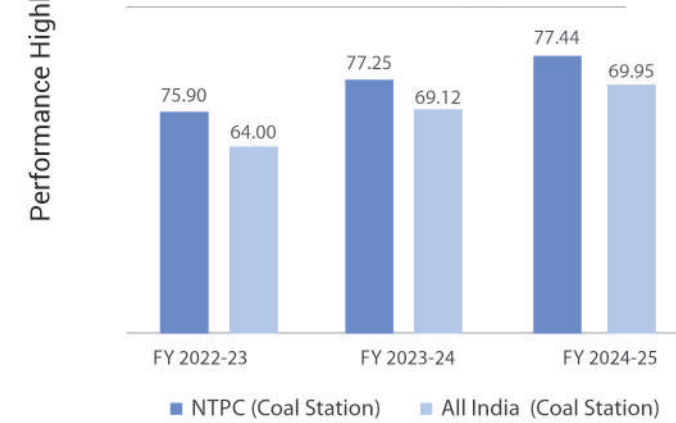
NTPC PLF Vs All India PLF (%)
